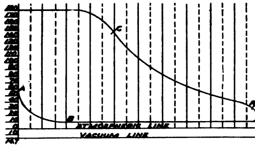
FIG. 231.—The Cycle of a Steam Engine, as shown by the Indicator Card. On this tracing, the admission is shown from A to C; the cut-off at C; the expansion curve from C to R; the release, or opening of the exhaust, at R, exhaust continuing from R to B; closing of the exhaust valve at B; compression of the residual steam in the cylinder clearance, from B to A. The figures on the left-hand vertical line indicate the gauge pressures. This diagram shows the operative conditions in a "high-pressure" cylinder; Fig. 232, in a "low-pressure" cylinder.
